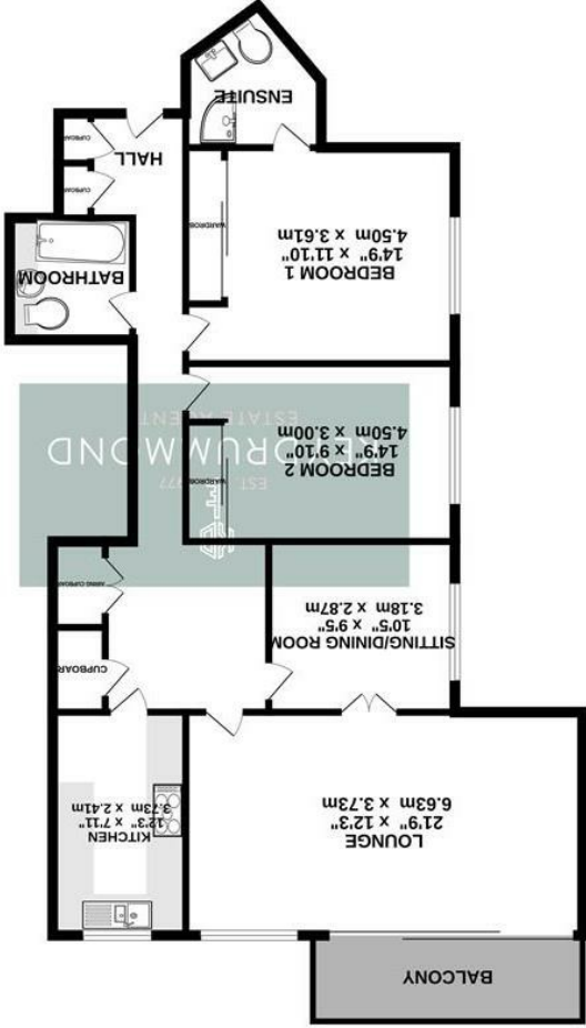
FLOORPLAN 1068 sq.ft. (99.2 sq.m.) approx.
